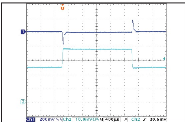
Figure 5: Output voltage response in the SM version to step-change in load current (50%-75%-50% of I_{out(max)} ; dI/dt = 0.1 A/\mu s ). Load cap: 100 \mu F electrolytic cap and 1 \mu F ceramic cap. Ch 1: V_{out} (200 mV/div), Ch 2: I_{out} (5 A/div).
